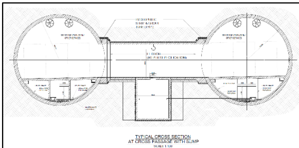
Figure 136: Typical Cross Section for Tunnel Cross Passage
