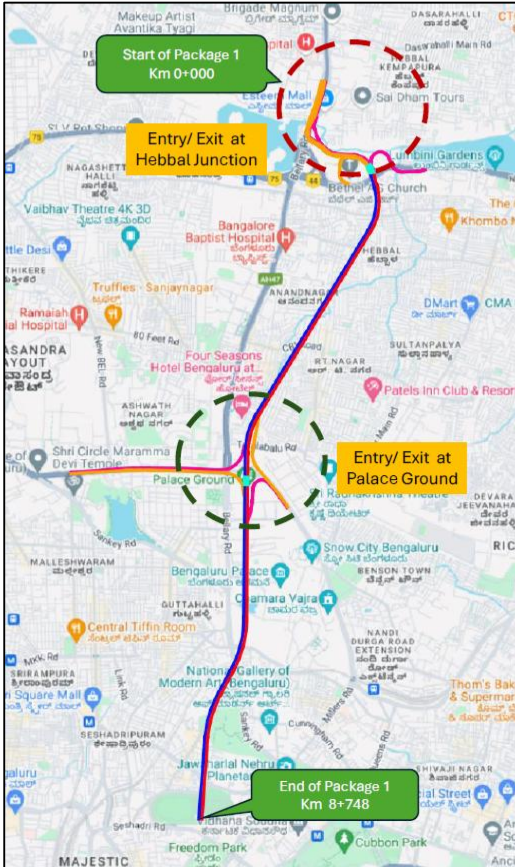
Figure 109: Package 1 Alignment
