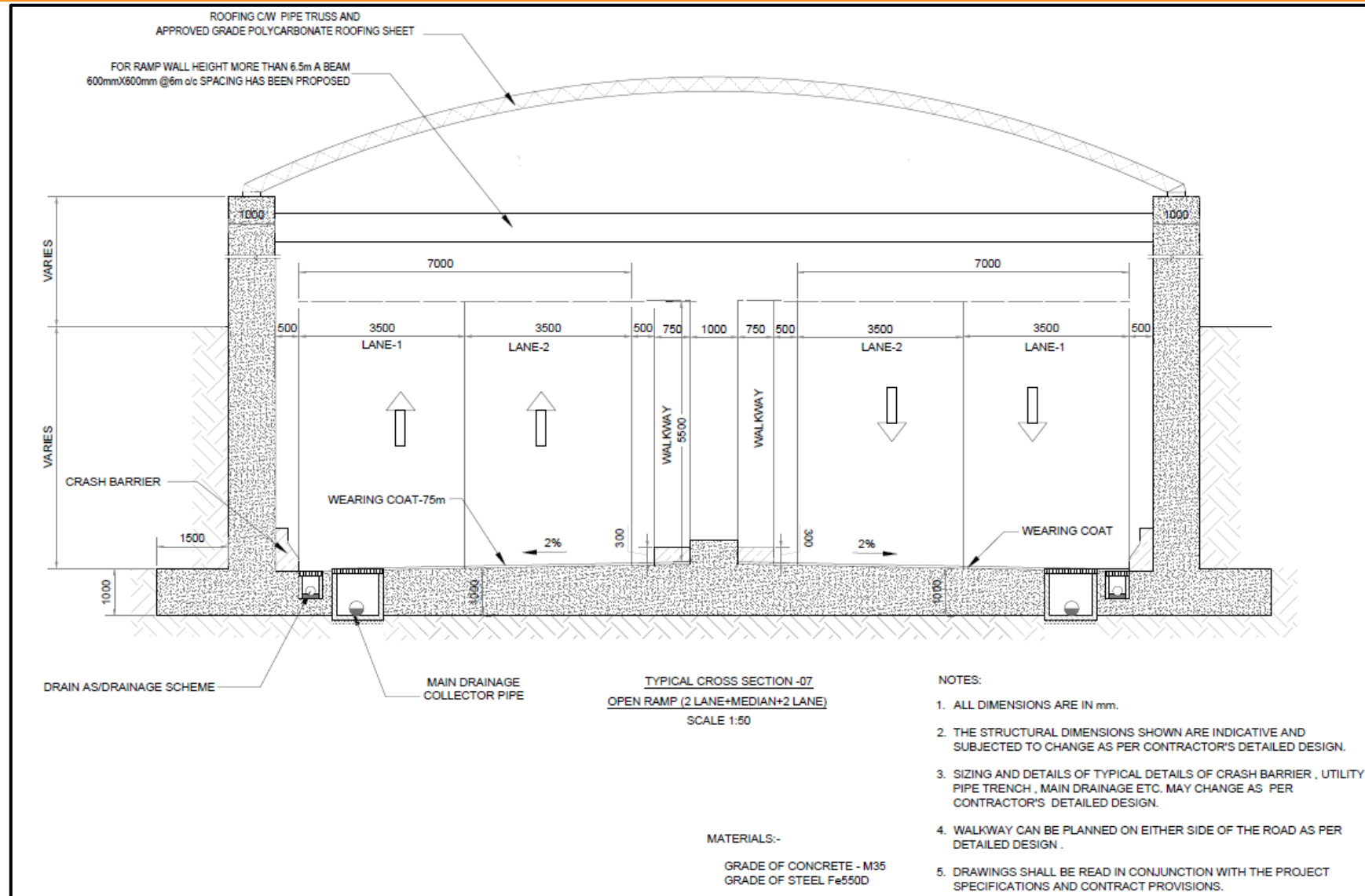
Figure 124: TCS-7, 2+2 lane Open Cut Section
