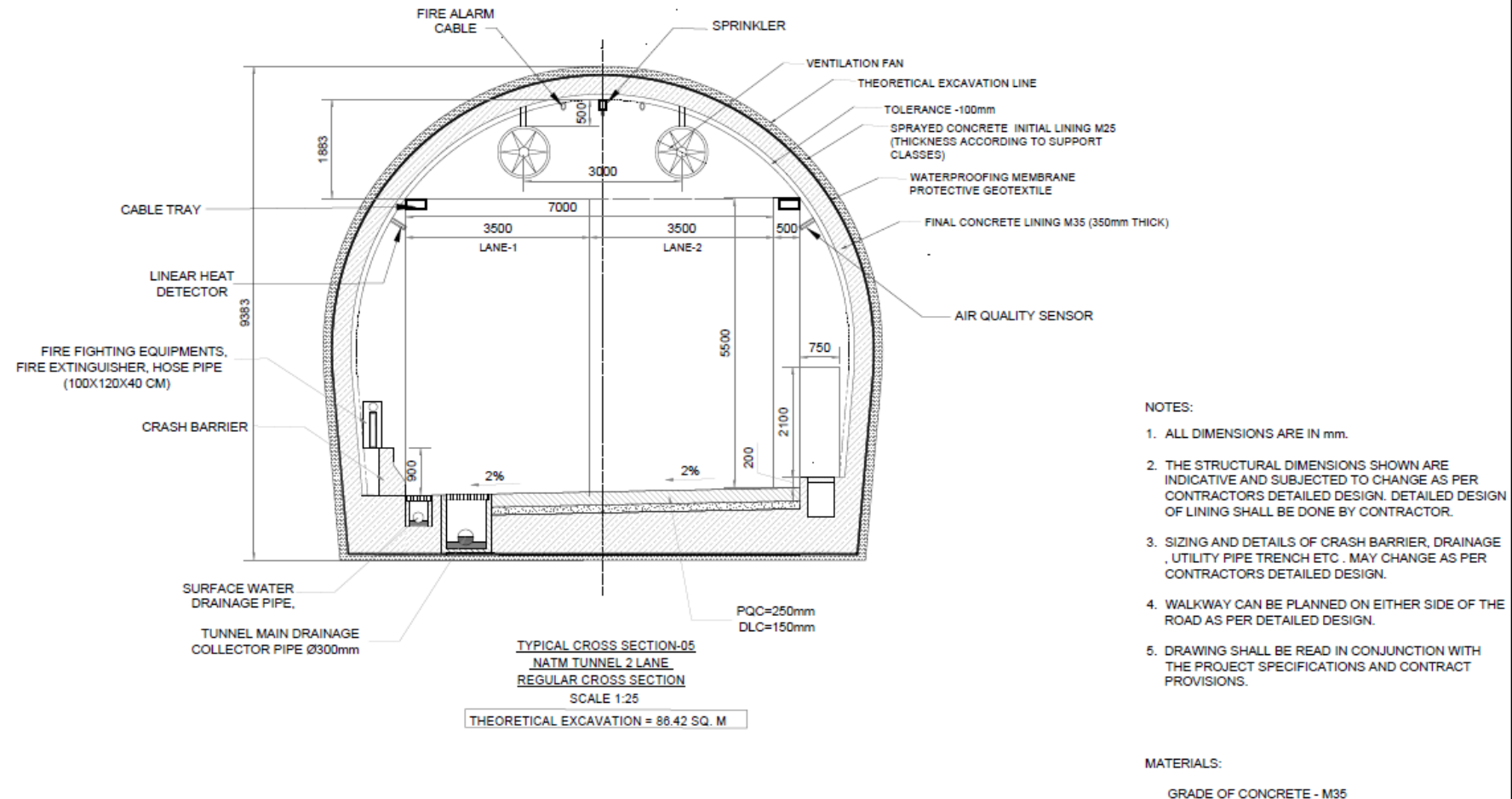
Figure 121: TCS-5, 2 Lane NATM Section
