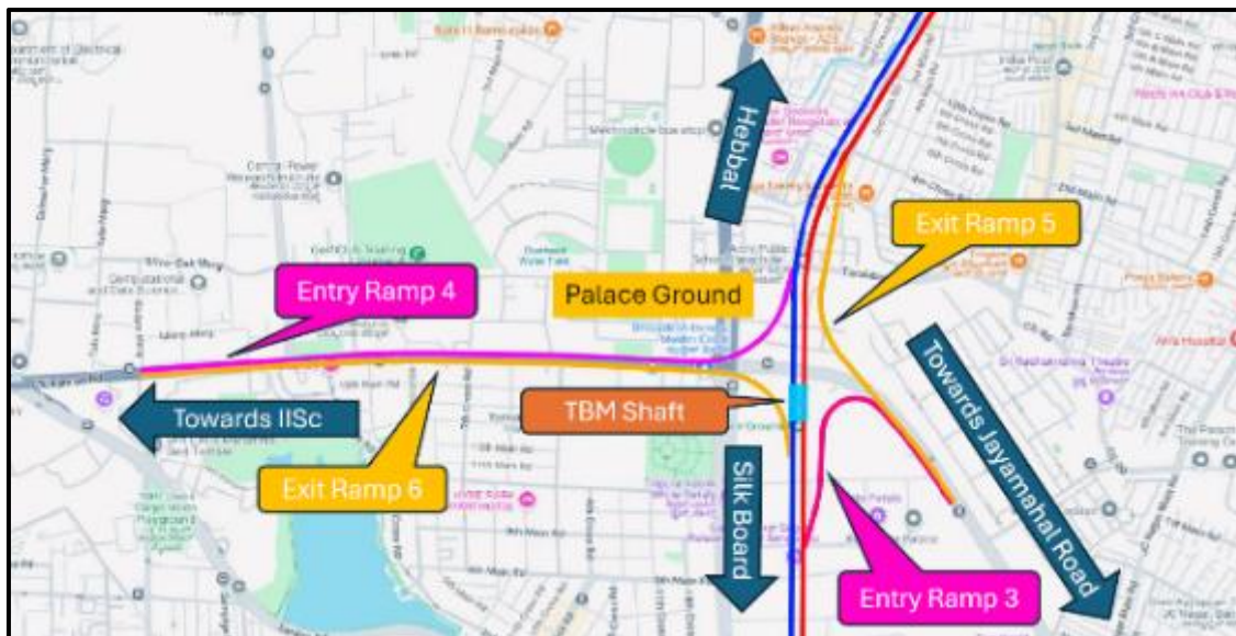
Figure 111: Ramps at Mekri Circle/Palace Ground
