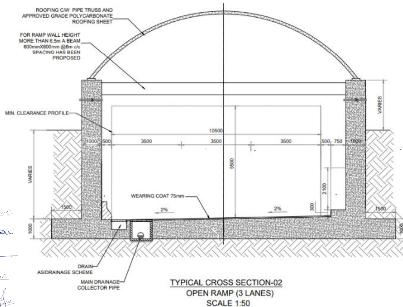
Figure 117: TCS-2, 3 lane Open Cut Section
